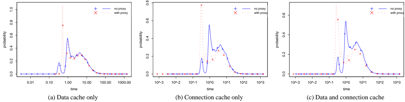
Fig. 6. Total latency comparison for AT&T WorldNet modem trace
