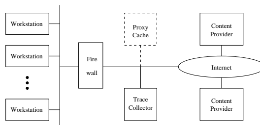
Fig. 2. Trace gathering environment for AT&T Labs-Research.
