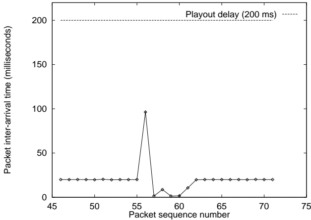
Figure 9: This graph shows packet interarrival times during a handoff, from a stream of UDP packets that mimics an audio stream. All packets arrived in order, without loss or duplication. The jitter added by the handoff is well below the limit imposed by the playout buffer at the receiver.
