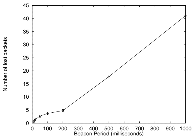
Figure 6: This graph shows the number of packets lost due to a handoff, when there is no buffering or retransmission, from a stream of UDP packets that mimics an audio stream.
