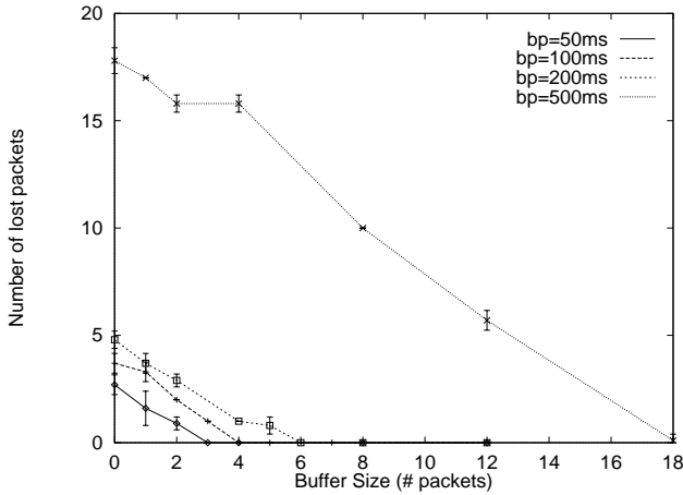
Figure 7: This graph shows the number of packets lost due to a handoff, from a stream of UDP packets that mimics an audio stream.
