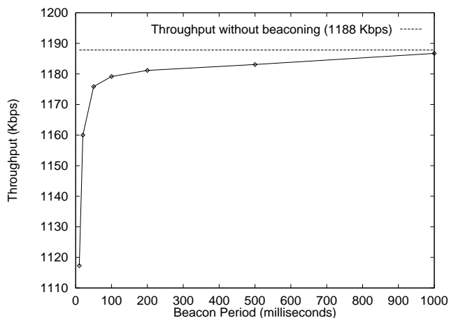
Figure 5: This graph shows the impact of beacons on TCP throughput, as measured by a ttcp receiver. Throughput begins to drop significantly when the beacon period drops below 50 ms.
