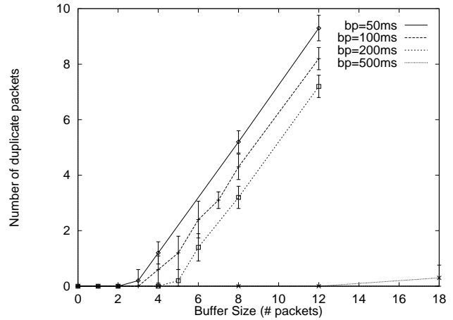
Figure 8: This graph shows the number of packets duplicated due to a handoff, from a stream of UDP packets that mimics an audio stream.
