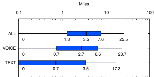
Figure 6. Comparison of the median daily ranges when considering only one event type. Voice calls have larger ranges than text. For clarity of display, we show only NY area on the weekdays in the winter. Other regions/times exhibit similar behavior.
