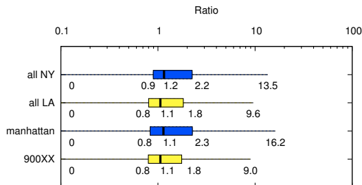
Figure 5. Ratio between median daily ranges weekday:weekend. The plot uses only the Winter dataset.
