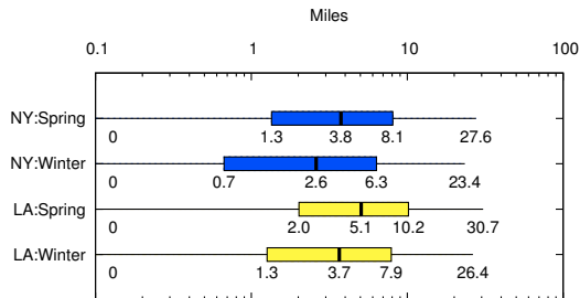
Figure 3. Median daily range in Spring and Winter for voice calls. Variations in median daily ranges between LA subareas span from 1.05 times at the 98 th percentile to 2.05 times at the 25 th percentile. Differences between NY subareas are even greater, spanning from 1.01 to 3.03 times at the 98 th and 25 th percentiles, respectively. One subarea from each city stands out. In NY, Manhattan tends to have significantly lower median daily ranges. This result is consistent with the idea that many people commute into the city center and those that already live there do not need to travel far. Conversely, in LA the outstanding region is Antelope Valley, which is on the outskirts. In this case, it appears that those who live far away from the city center tend to commute much further.
